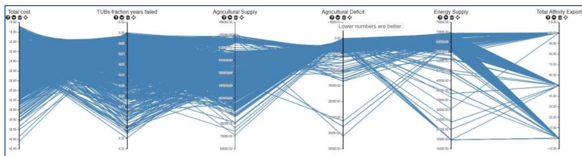
Figure 39: PolyVis tool
